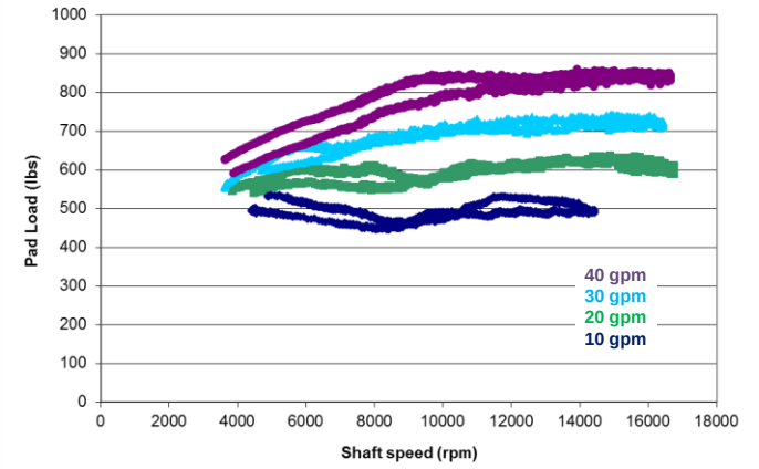
Figure 23: Offset Pivot Direct Lube with O-Ring, Pad Load vs Speed.
