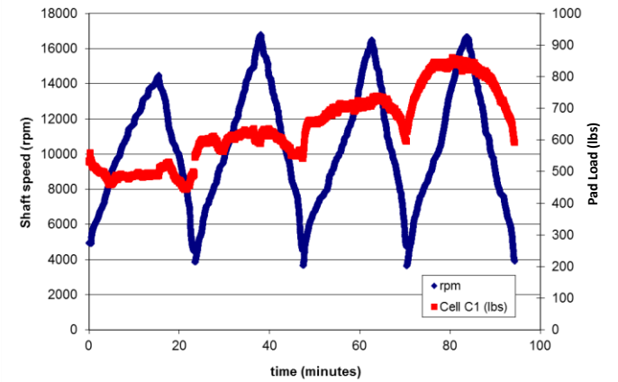
Figure 22: Offset Pivot Direct Lube with O-Ring, Pad Load vs Time.
