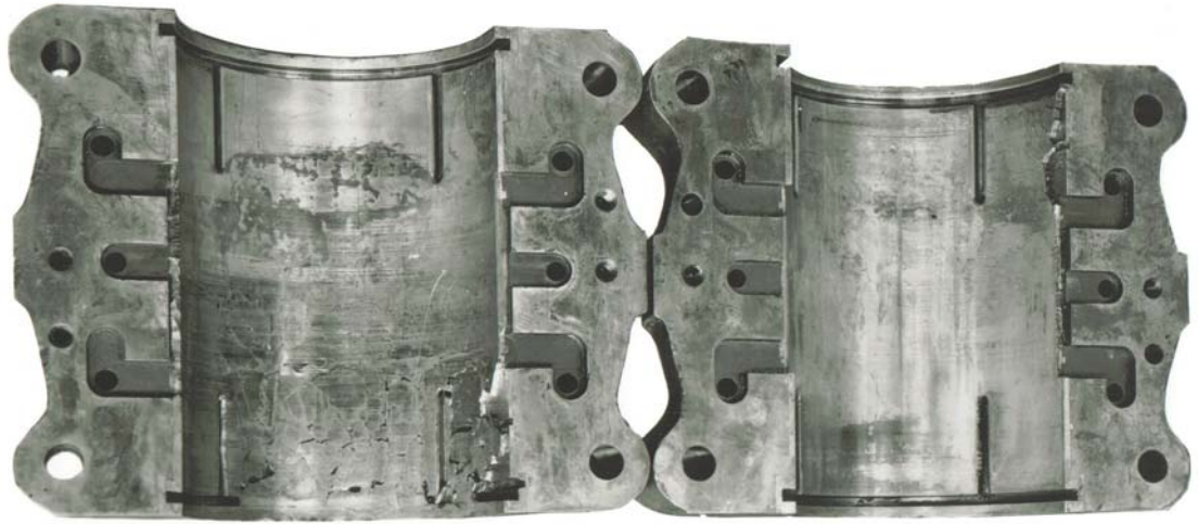
Figure 26 Edge Load Journal Shell With Babbitt Mechanical Fatigue
