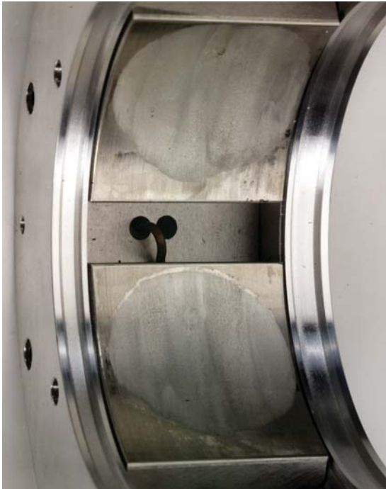
Figure 24 Stray Shaft Currents/ Electrical Pitting (Frosting)
