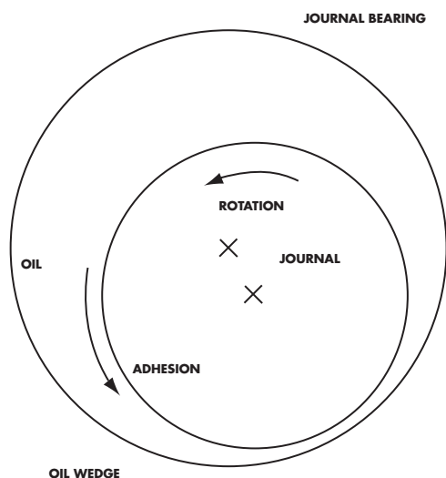
Figure 4 Hydrodynamic Principle
