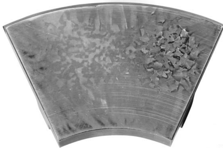
Figure 17 Thermal Ratcheting
