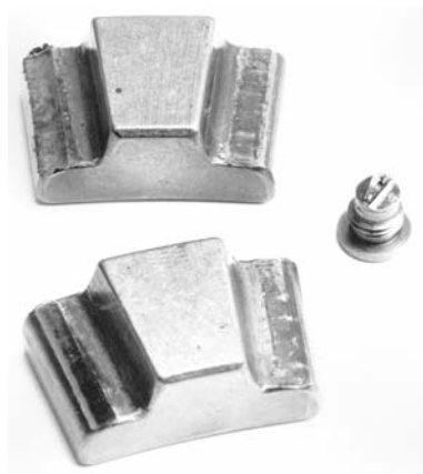
Figure 36 Leveling Plate Wear Due To Collar Wobble
