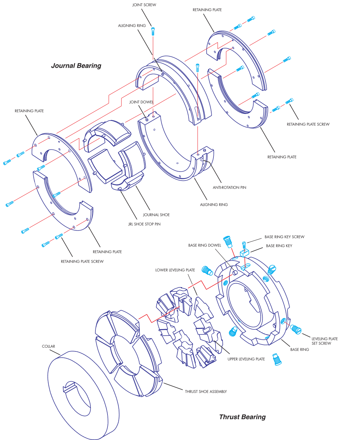
Figure 7 Thrust and Journal Bearing Part Schematic
