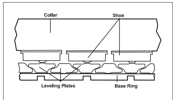
Figure 8-2 Thrust Bearing Load Equalization and Alignment Features
