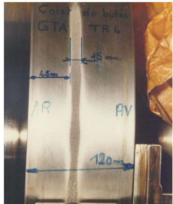
Figure 33 Cavitation Damage on Outside Diameter of Collar
