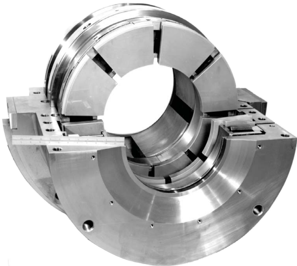
Figure 3 Hydrodynamic Tilting Pad Thrust and Journal Bearing
