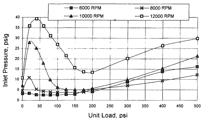
Figure 5. Standard LEG Oil Supply Pressure for Recommended Flowrate.
