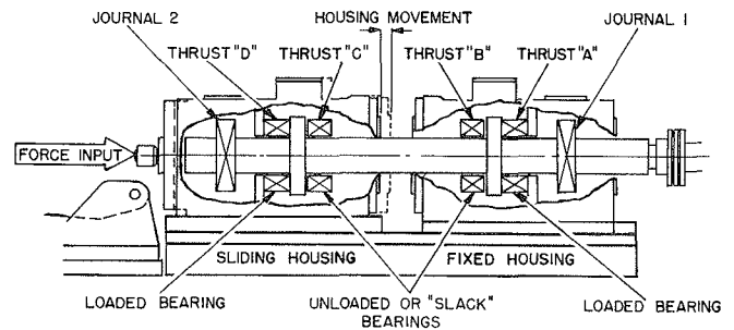
Figure 1. Bearing Arrangement Within Test Housings.
