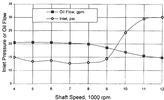
Figure 7. Standard LEG Oil Supply Pressure and Flowrate Versus Shaft Speed for Fixed Valve Test at 50 PSI Unit Load.
