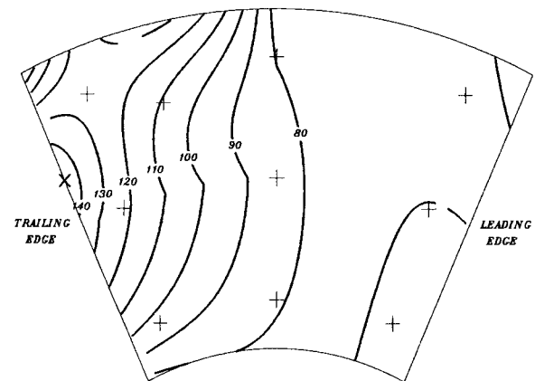
c) 115 m/s, T_{75/75} = 109^\circ\text{C} , T_{\max} = 147^\circ\text{C}
