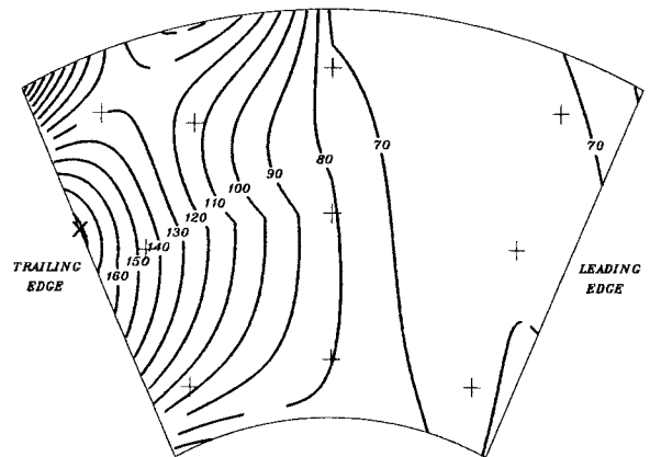
b) 94 m/s, T_{75/75} = 113^\circ\text{C} , T_{\max} = 182^\circ\text{C}
