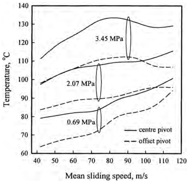
Fig. 13 Averaged pad temperature T_{75/75} , 267 mm o.d. bearing with offset and centre-pivot pads, ISO VG32 oil
