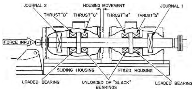
Fig. 2 Schematic of 267 mm o.d. thrust bearing test rig
