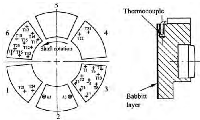
Fig. 3 (a) Instrumentation of the 228 mm o.d. bearing and (b) thermocouple mounting in the bearing pad
