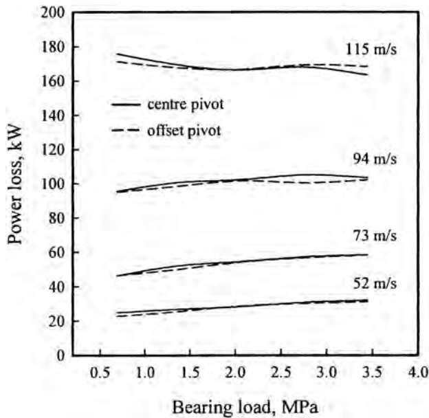
Fig. 15 Power loss, 267 mm o.d. bearing with offset and centre-pivot pads, ISO VG32 oil
