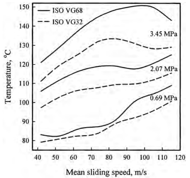
Fig. 6 Averaged pad temperature T_{75/75} , 267 mm o.d. bearing
