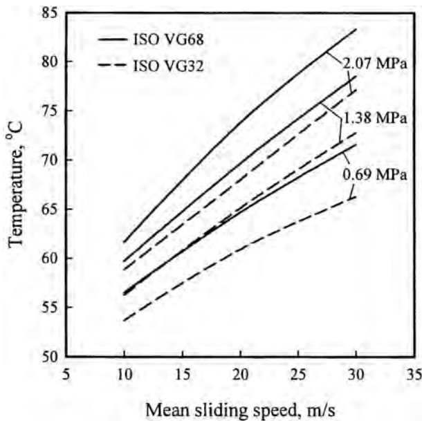
Fig. 5 Collar temperature T_{75} , 228 mm o.d. bearing
