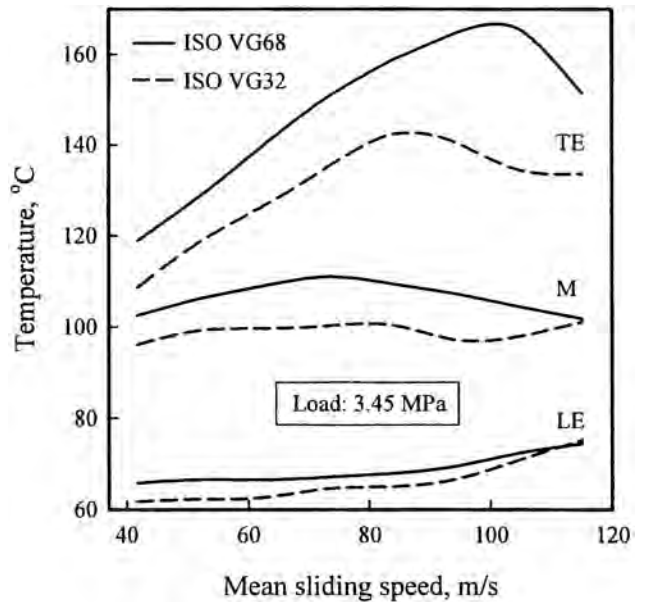
Fig. 7 Centre-line leading edge (LE), middle (M) and trailing edge (TE) temperatures, 267 mm o.d. bearing
