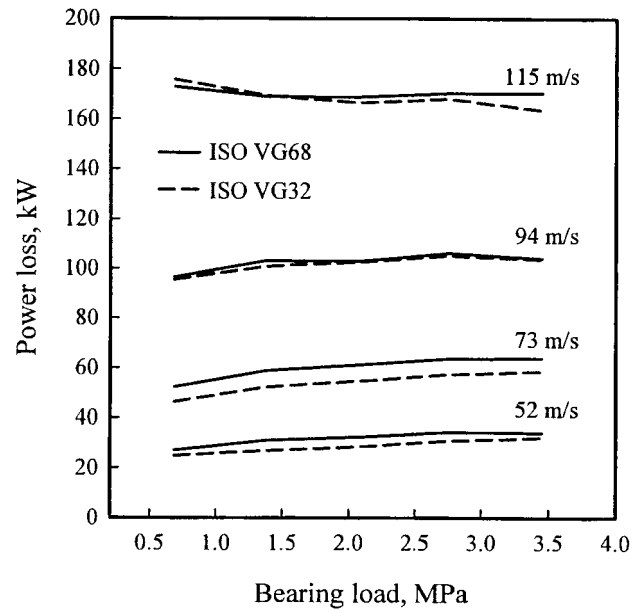
Fig. 10 Power loss, 267 mm o.d. bearing
