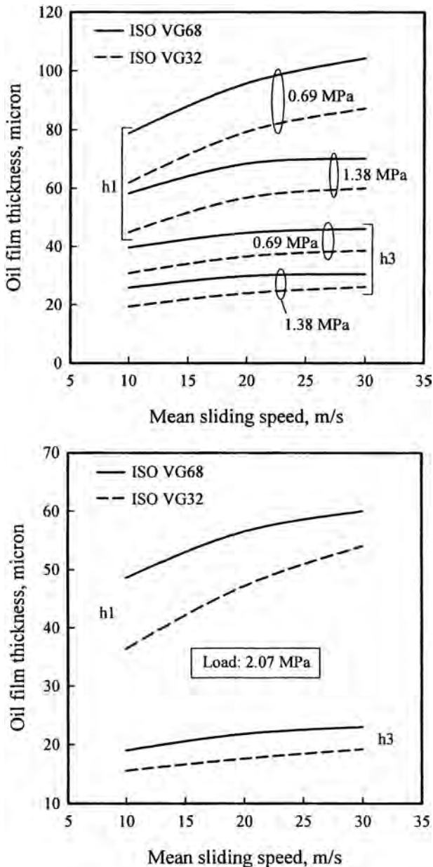
Fig. 11 Oil film thickness
