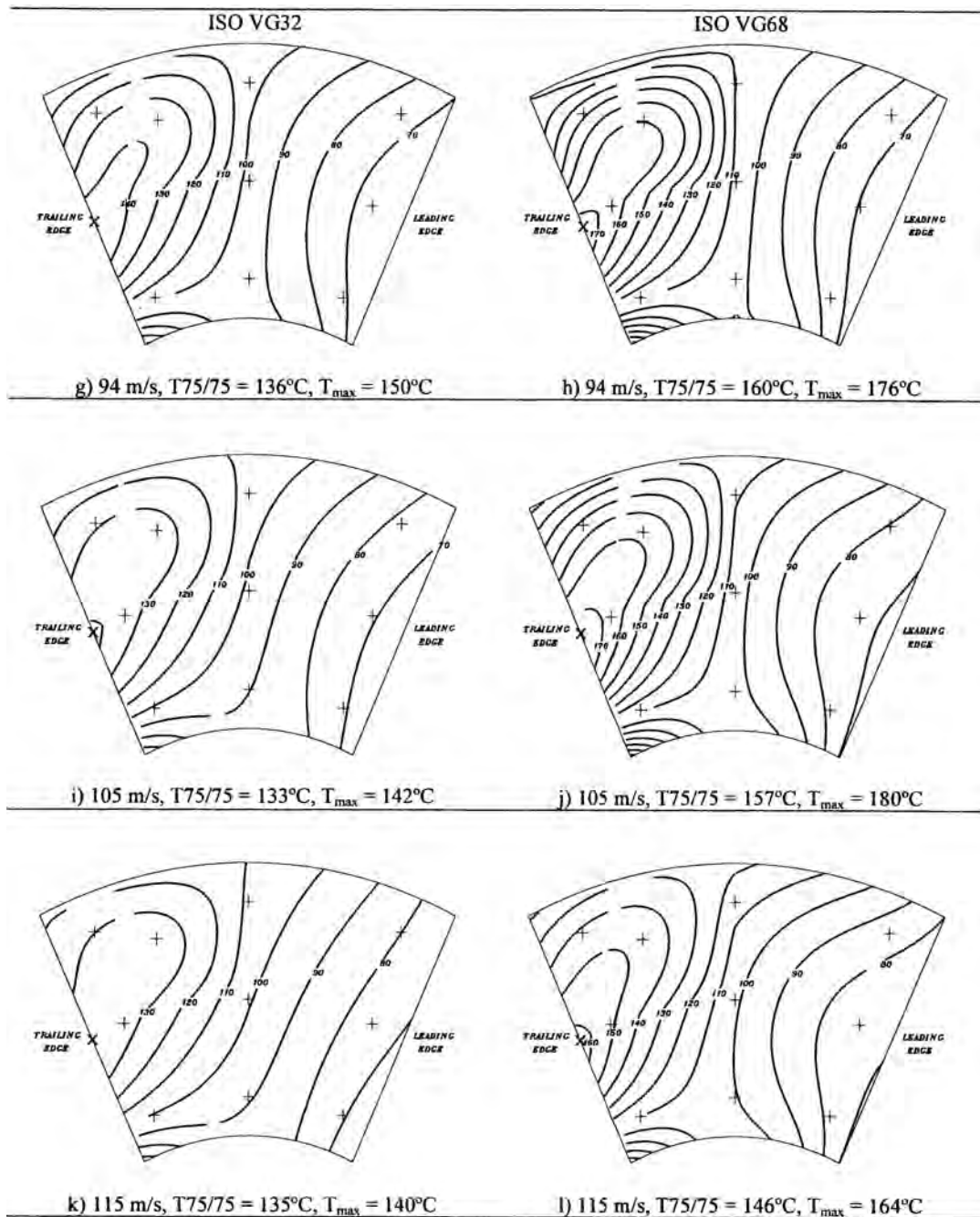
Fig. 12 Pad temperature patterns, 267 mm o.d. bearing, centre-pivot pad
