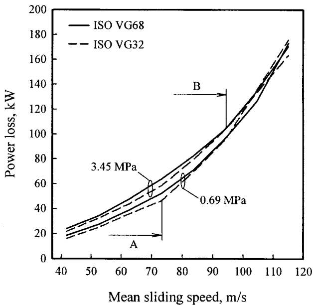
Fig. 9 Power loss, 267 mm o.d. bearing
