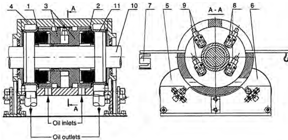
Fig. 1 Schematic of 228 mm o.d. thrust bearing test rig
