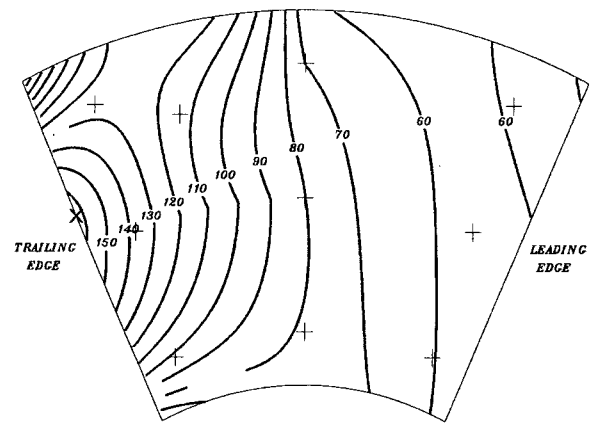
a) 73 m/s, T_{75/75} = 114^\circ\text{C} , T_{\max} = 164^\circ\text{C}
