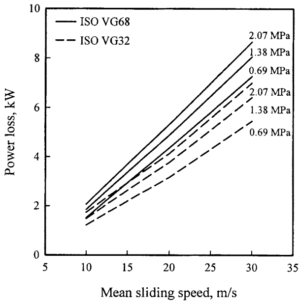
Fig. 8 Power loss, 228 mm o.d. bearing
