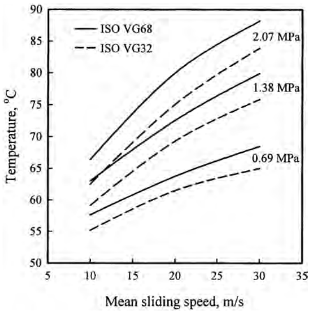
Fig. 4 Averaged pad temperature T_{75/75} , 228 mm o.d. bearing
