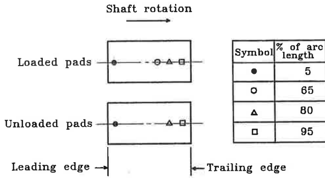
Fig.1 Thermocouple locations
