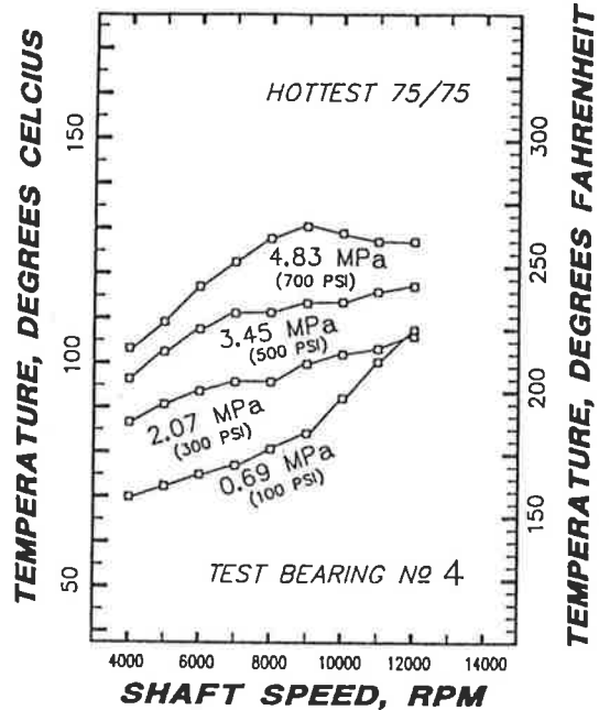
Fig. 11—A comparison of the hottest measured 75/75 percent babblitt temperature locations for test bearing No. 4 (99 percent CU + Ag + Mn + Se) when loaded with four tested loads at shaft speeds of 4000 to 12 000 RPM.
