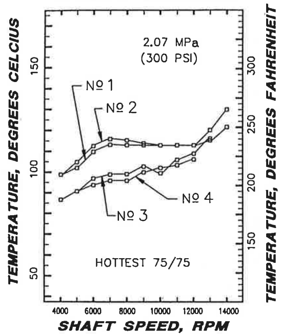
Fig. 5—A comparison of the hottest measured 75/75 percent babbitt temperature locations for each of the four shoe construction materials when loaded to 2.07 MPa at shaft speeds of 4000 to 14 000 RPM.
