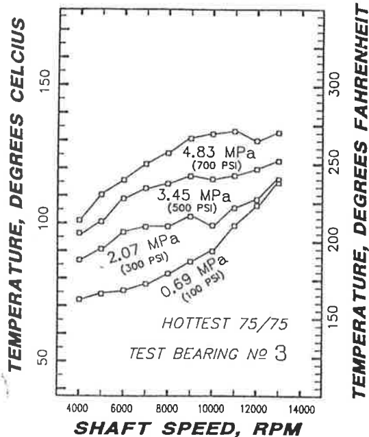
Fig. 10—A comparison of the hottest measured 75/75 percent babblitt temperature locations for test bearing No. 3 (93 percent CU + CR) when loaded with four tested loads at shaft speeds of 4000 to 13 000 RPM.
