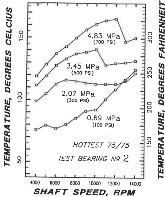
Fig. 9—A comparison of the hottest measured 75/75 percent babblitt temperature locations for test bearing No. 2 (70 percent CU + Pb + Sn) when loaded with four tested loads at shaft speeds of 4000 to 14 000 RPM.
