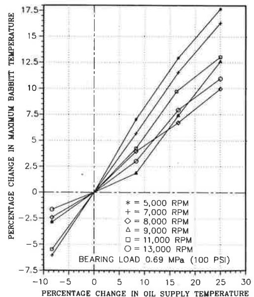
Fig. 3—A comparison of the percentage changes in maximum babbitt temperature for a percentage change in oil supply temperature for a bearing loaded to 0.69 MPa for shaft speeds of 5, 7, 8, 9, 11, and 13 000 rpm.
